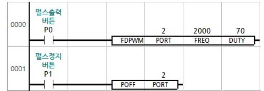
[ FDPWM 평선블럭 ]
