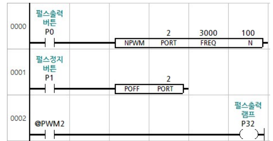
[ NPWM 평선블럭 ]
