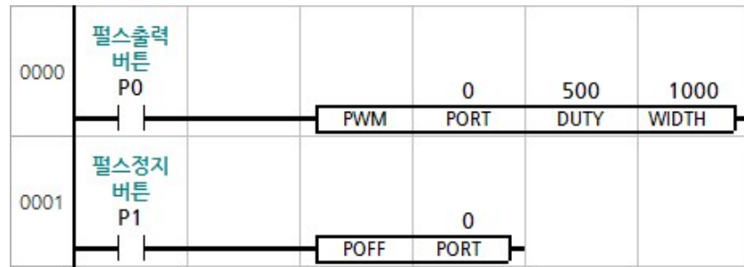
[ PWM 평선블럭 ]
